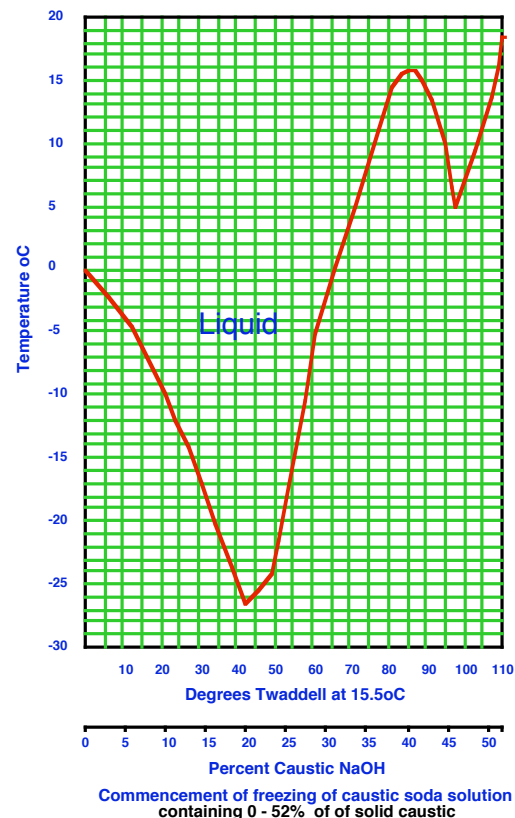
Graph Showing the Freezing Point of Caustic
